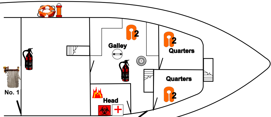
Main Deck
