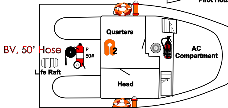
01 Deck Layout
